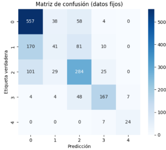
(a) ViT-B/16 (google/vit-base-patch16-224)
