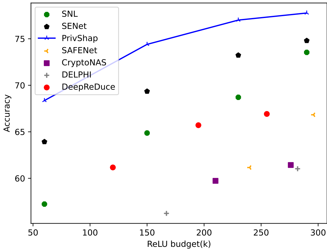
CIFAR-100
