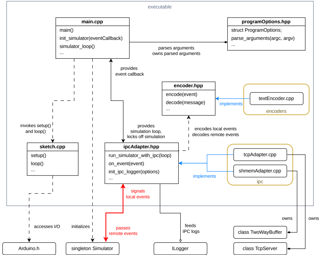
Figure 3.2 executable module architecture
