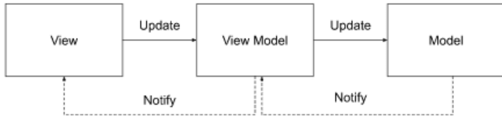
Figure 2.5 MVVM architecture [7]
