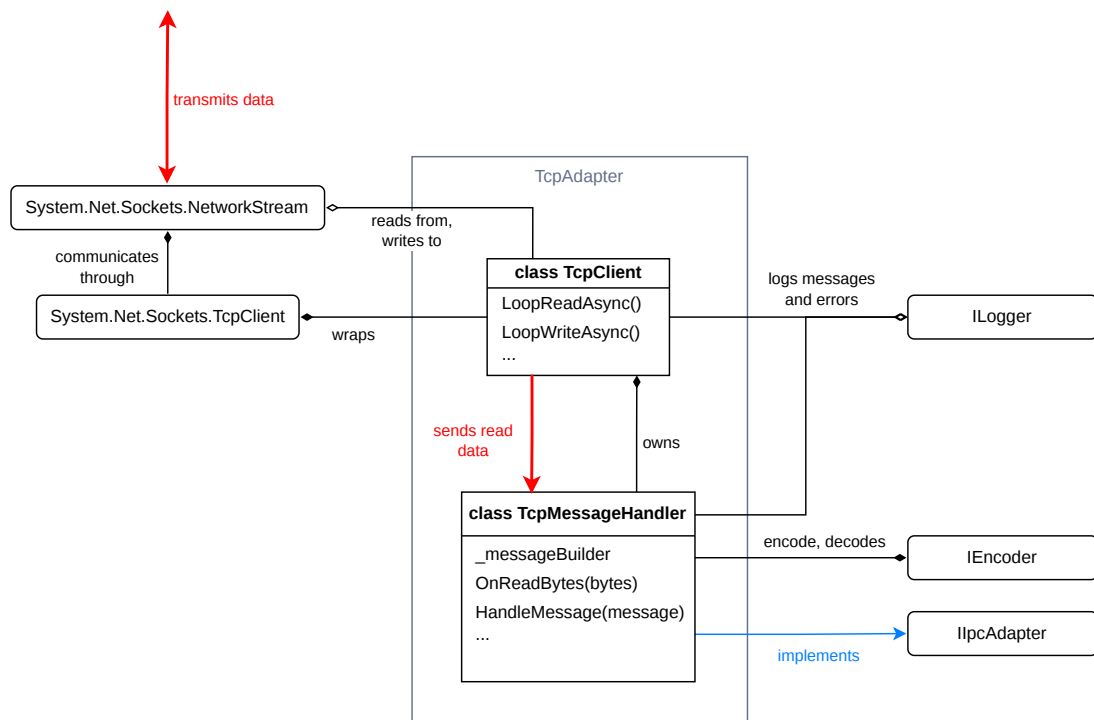
Figure 4.5 tcpAdapter project architecture
