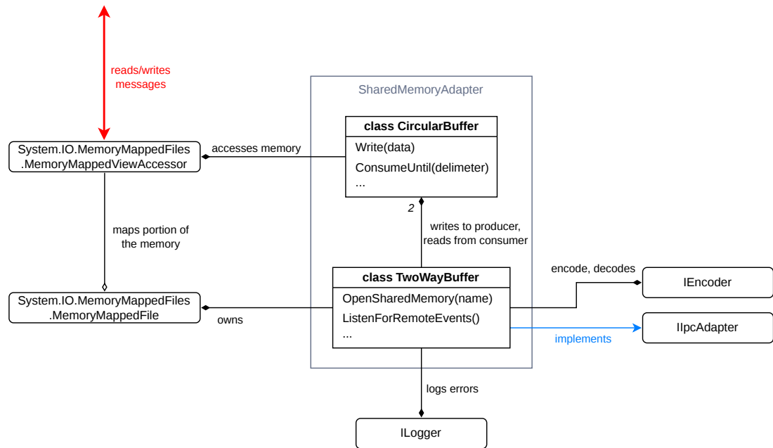
Figure 4.6 SharedMemoryAdapter project architecture
