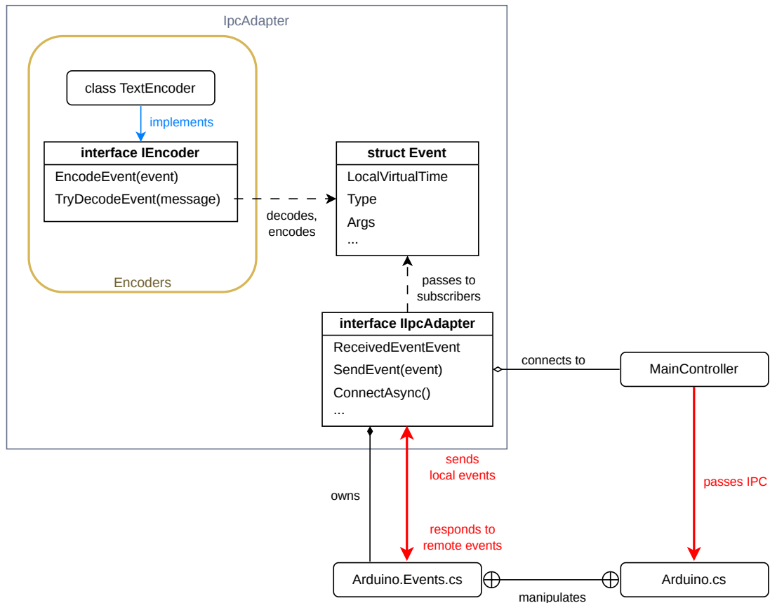
Figure 4.4 IpcAdapter project architecture
