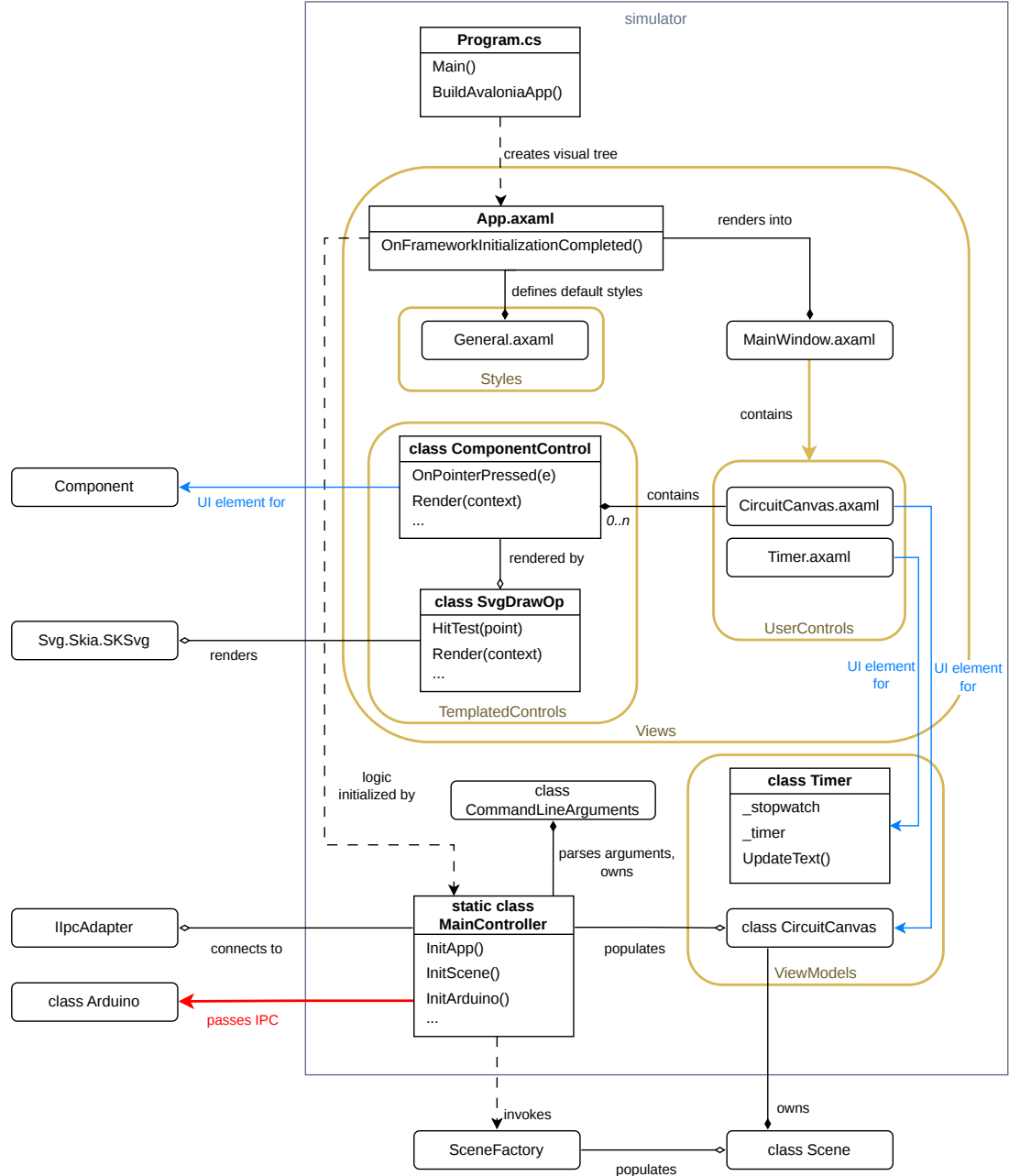
Figure 4.3 Main project architecture
