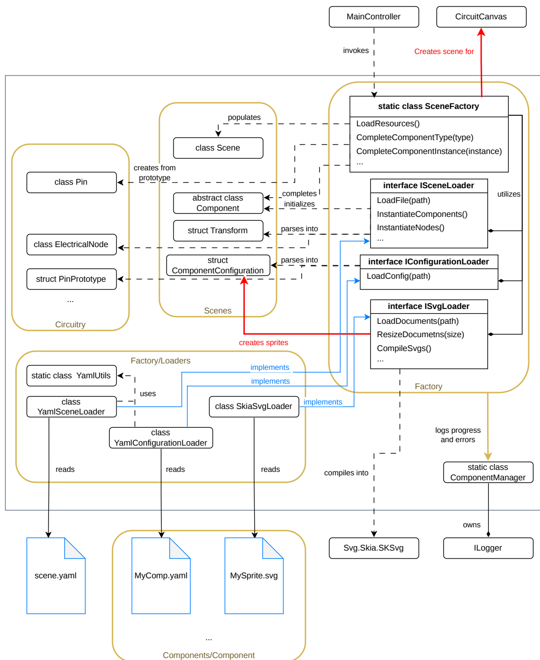
Figure 4.2 Factory architecture of the ComponentManagement project
