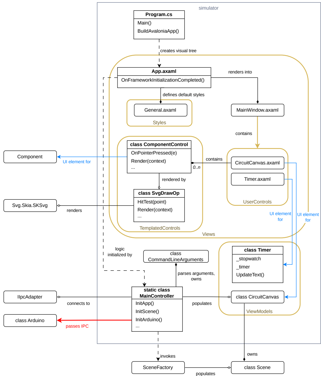
Figure 4.3 Main project architecture GeometryExtensions missing
