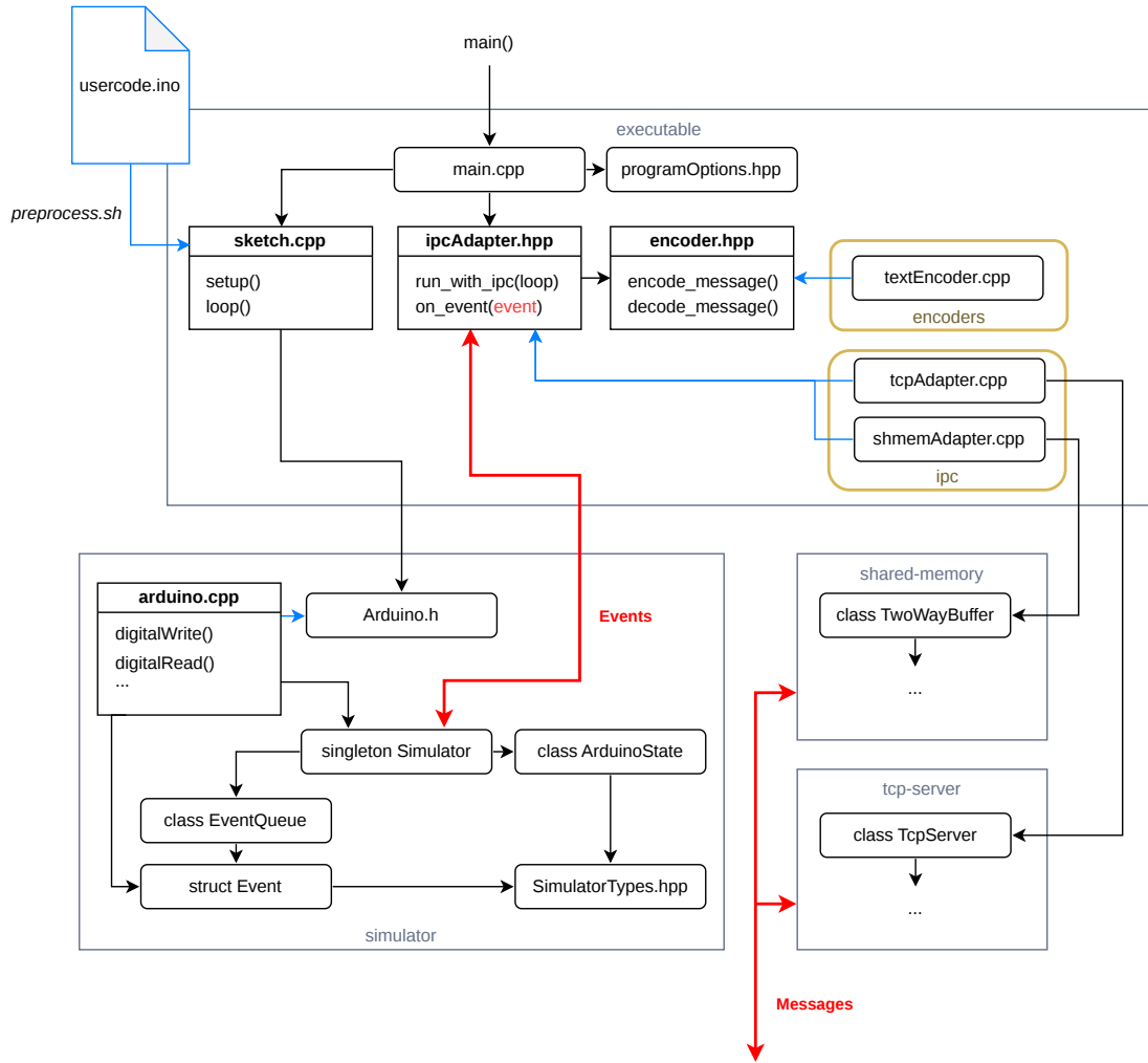
Figure 2.3 Backend architecture
