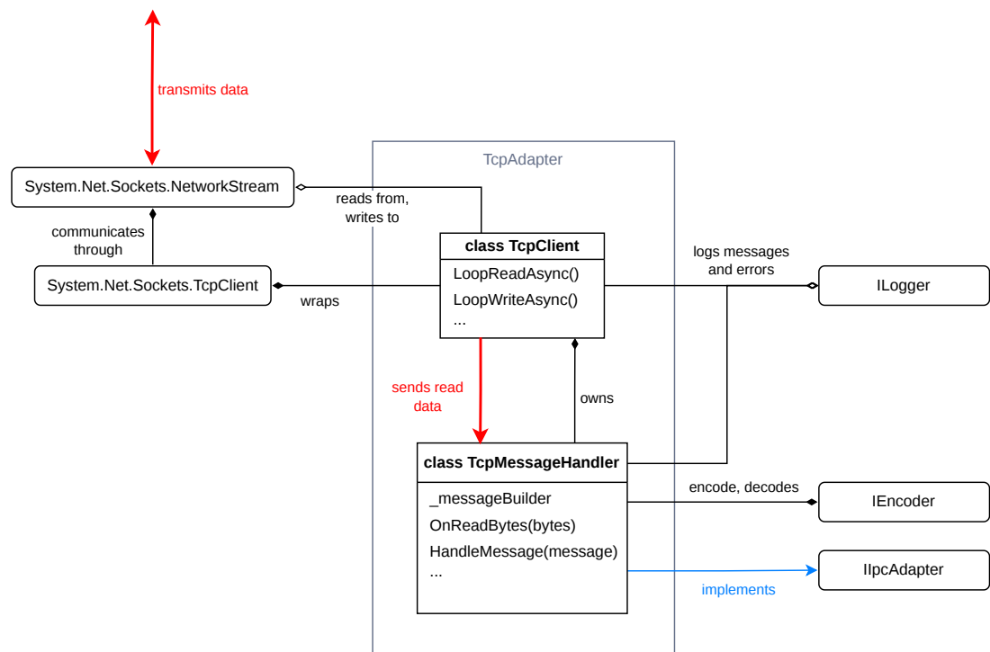
Figure 4.6 tcpAdapter project architecture
