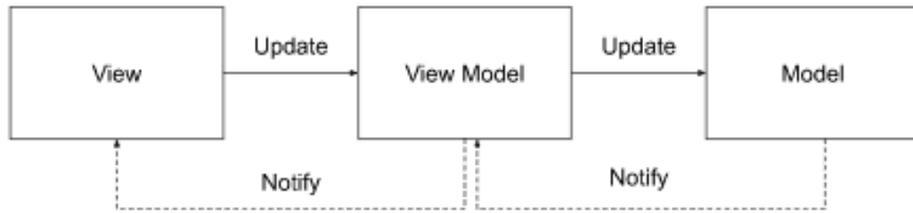
Figure 1.5 MVVM architecture [3]
