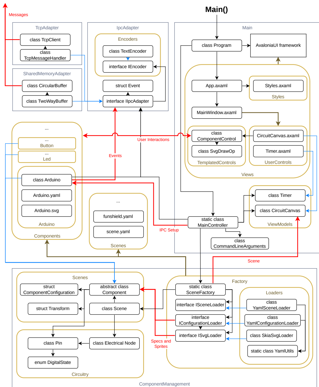
Figure 2.4 Frontend architecture
