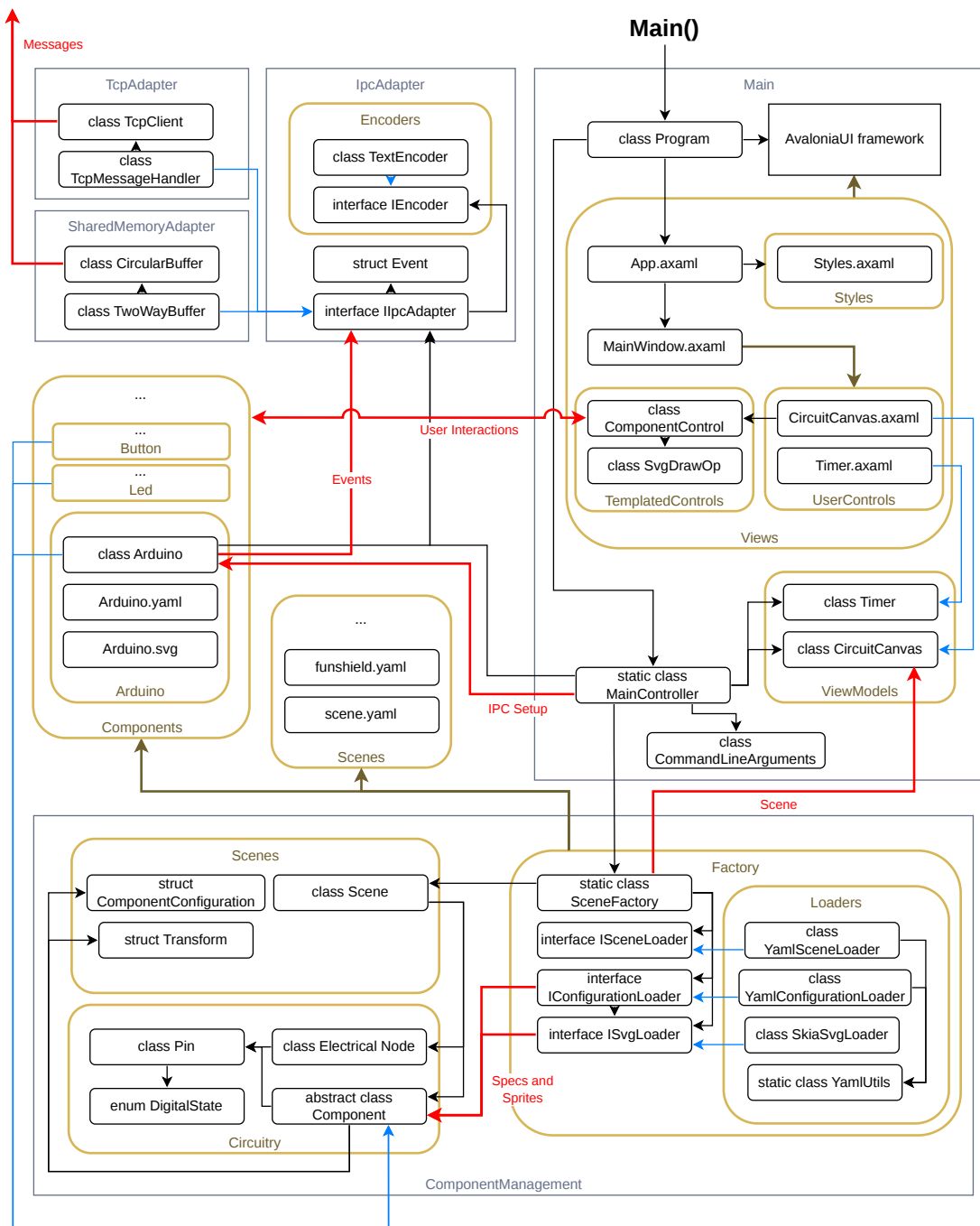
Figure 1.3 Frontend architecture
