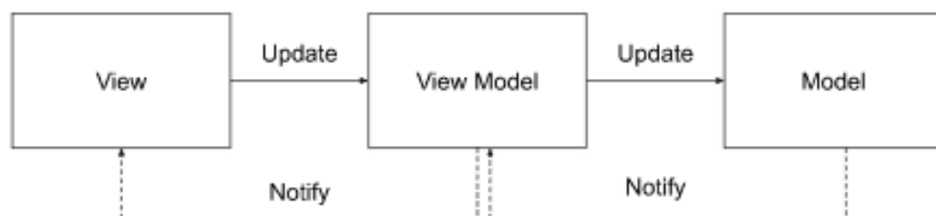
Figure 1.4 MVVM architecture [2]
