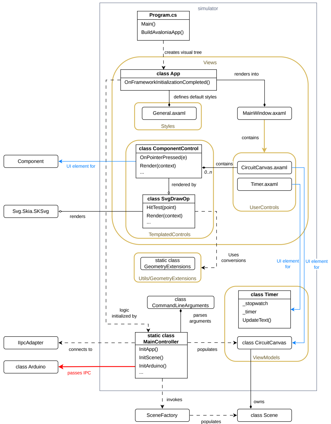
Figure 4.3 Main project architecture
