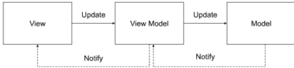
Figure 2.5 MVVM architecture [7]
