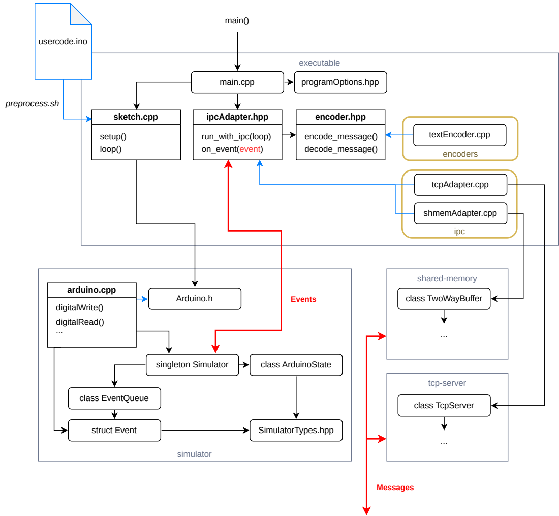
Figure 2.3 Backend architecture
