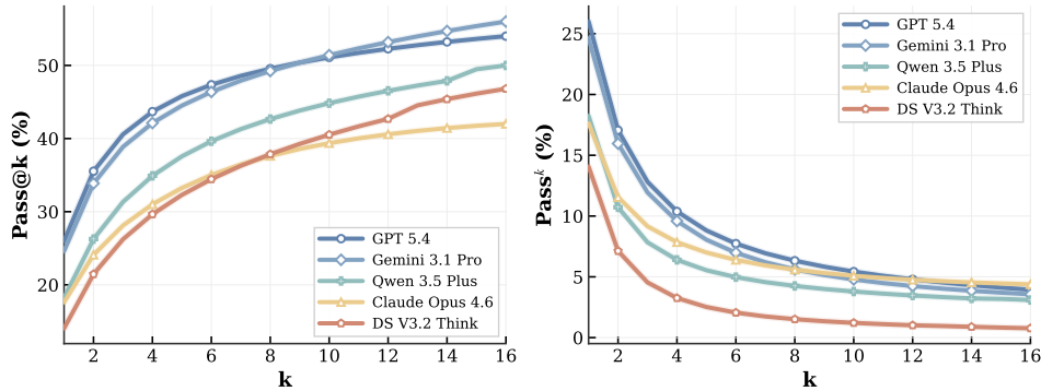
Figure 10: Model performance under Pass@k and Pass k .
