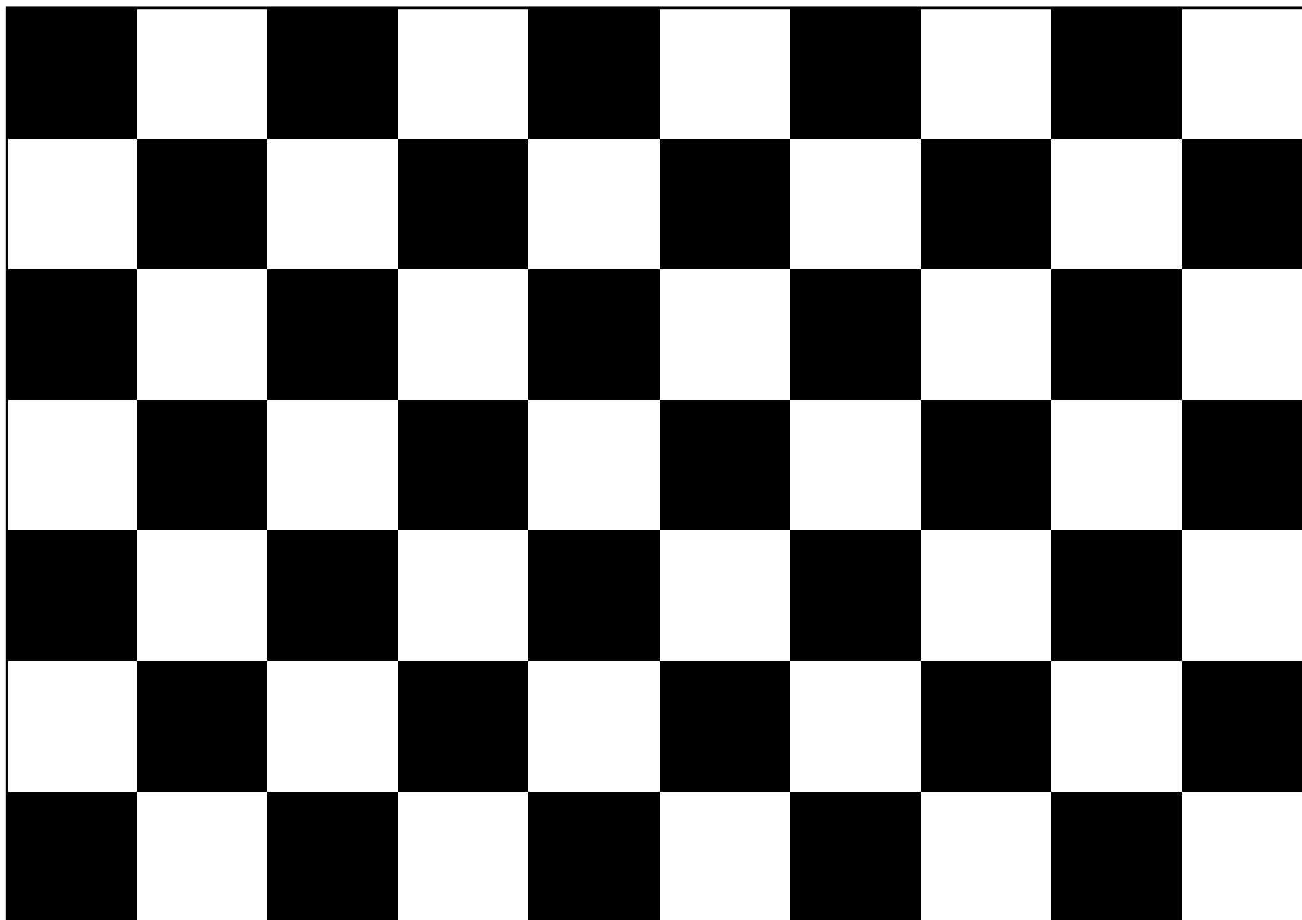
Chessboard Calibration Pattern: 9x6 inner corners | Square size: 25mm Print at 100% scale (no fit-to-page) | A4 Landscape
