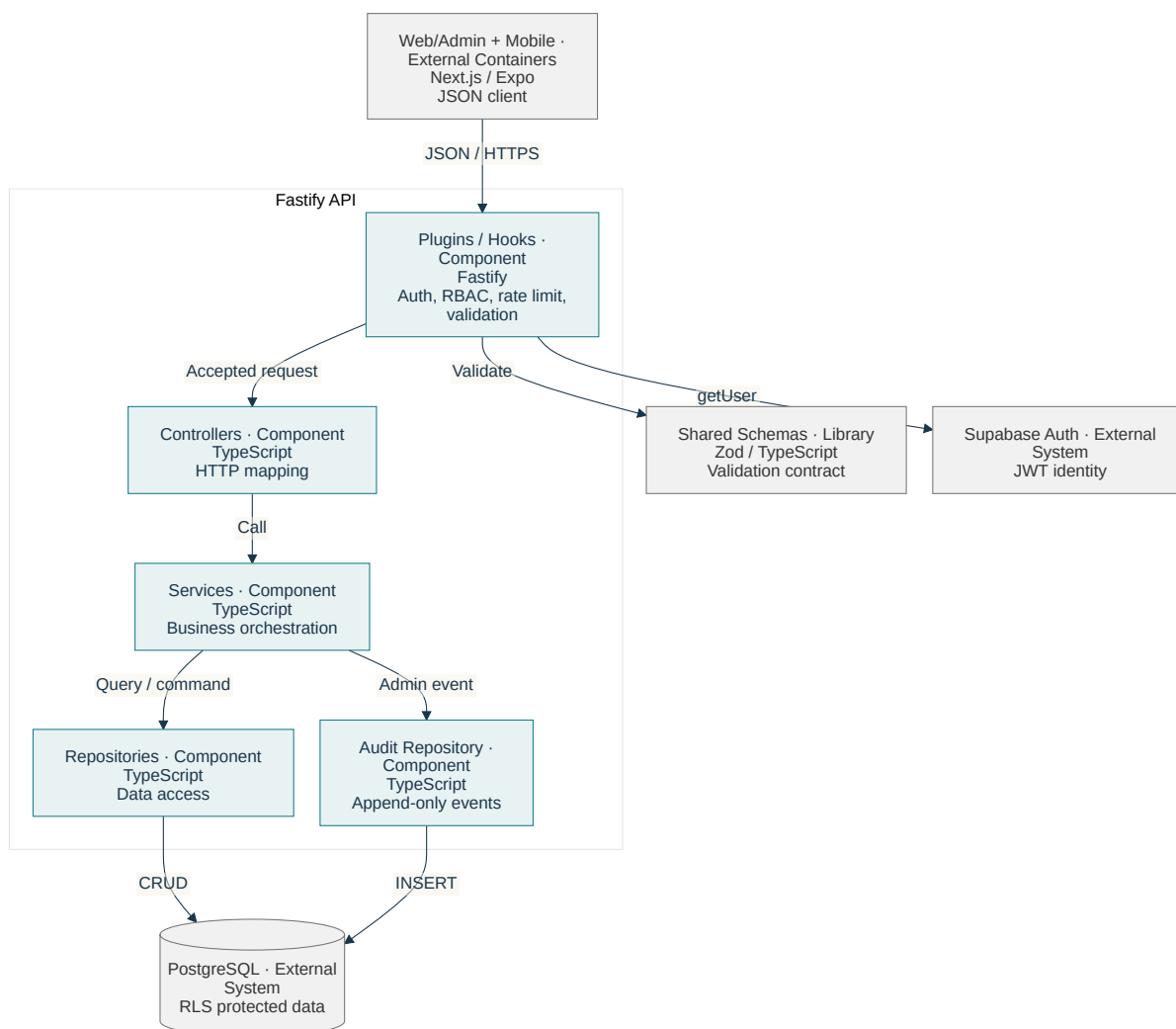
Зураг 3: C4-03 — Fastify API Component View
