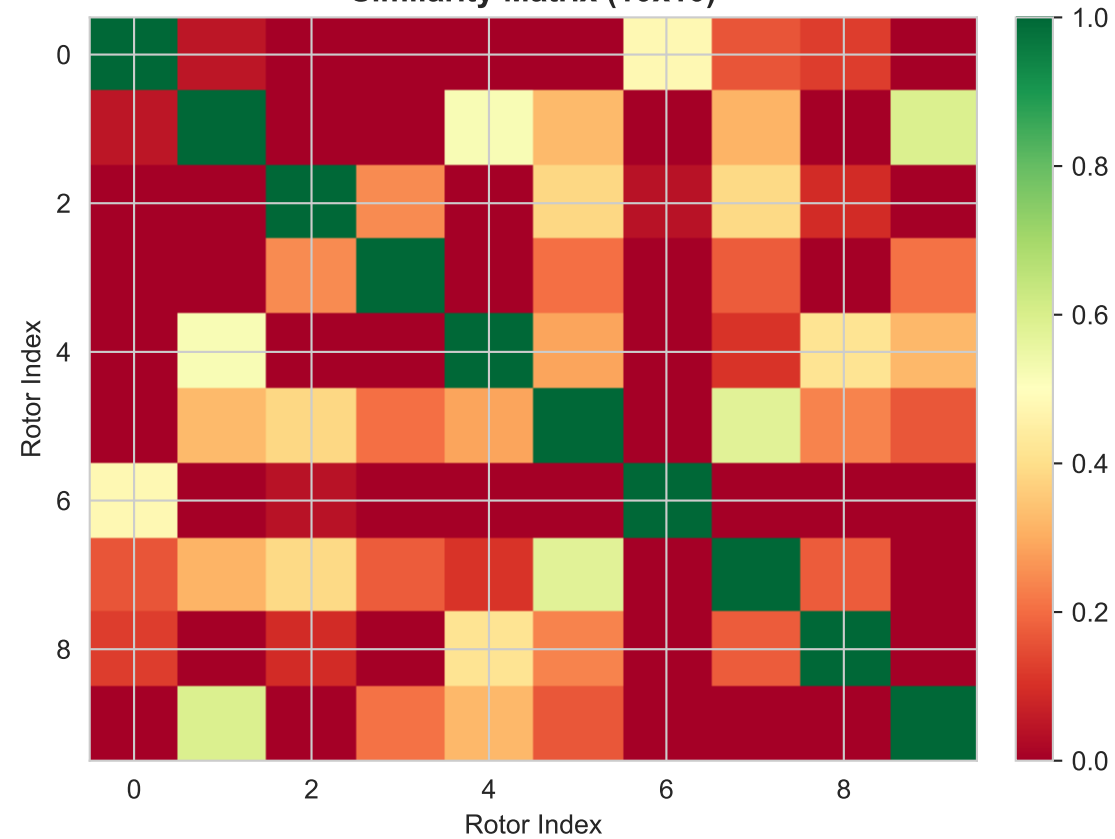
Autoencoder Similarity Matrix (10x10)
