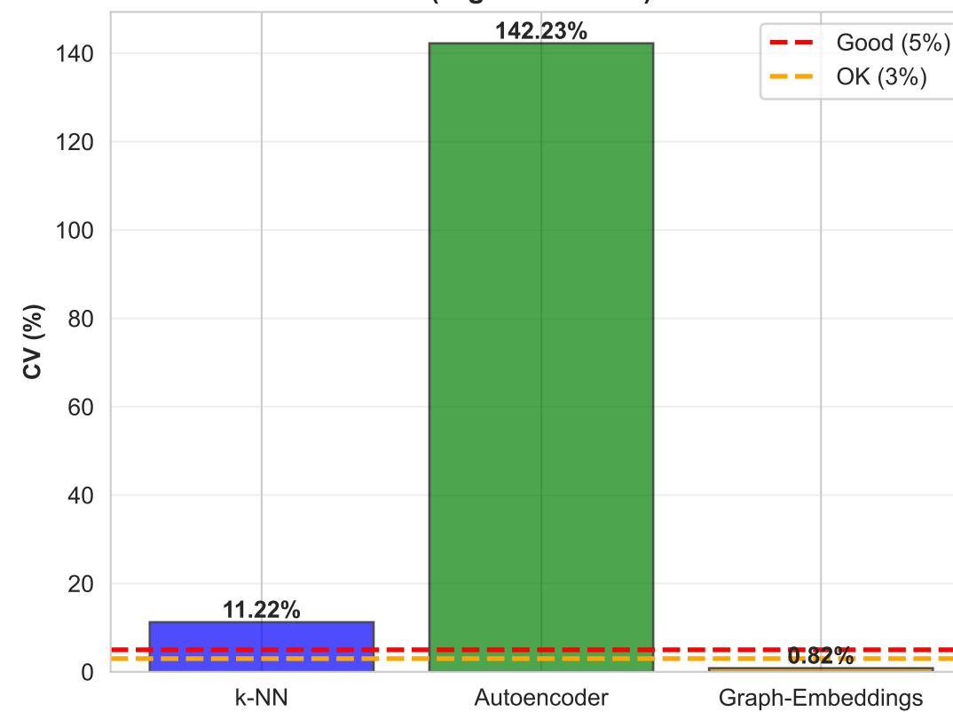
Coefficient of Variation (Higher = Better)
