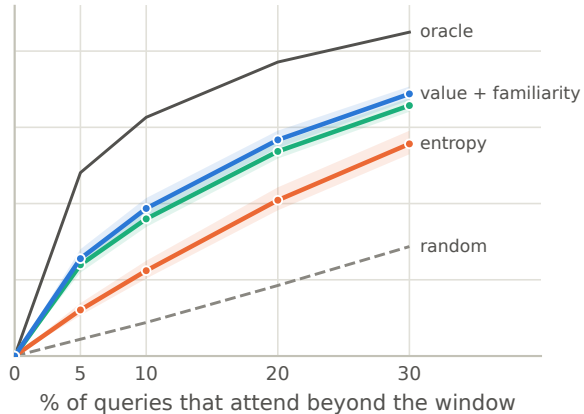
(b) Qwen2.5-7B · 8k context · window 1024
