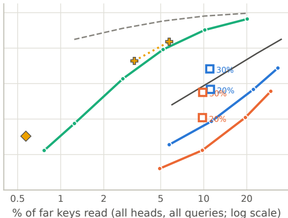
Qwen2.5-7B · 8k context · window 1024
