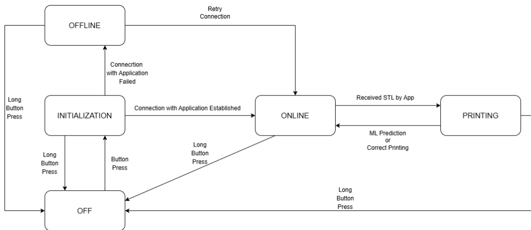
Actuator State Diagram
