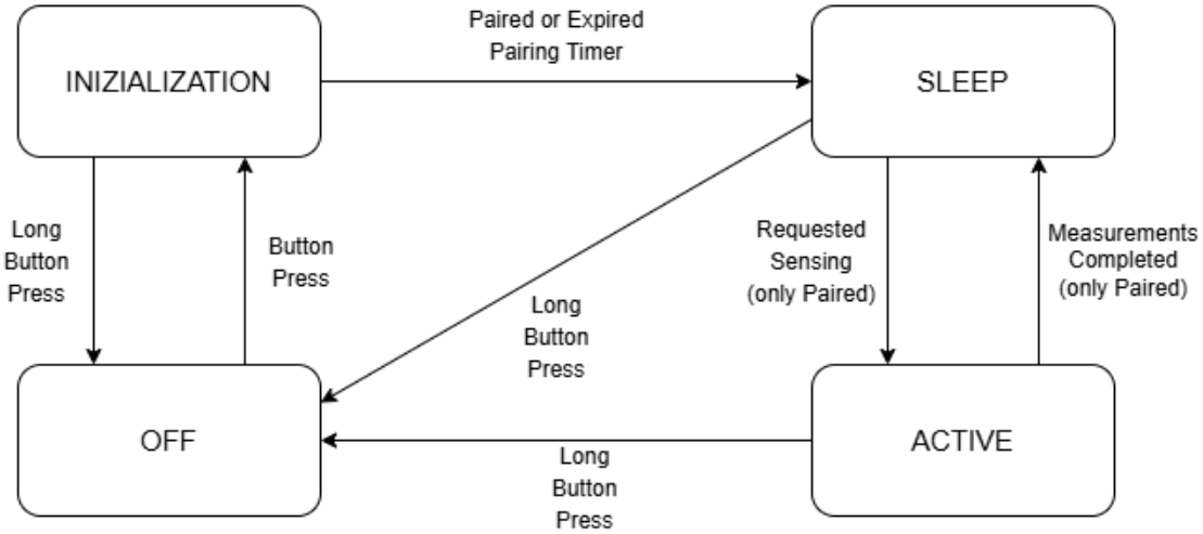
Sensor State Diagram
