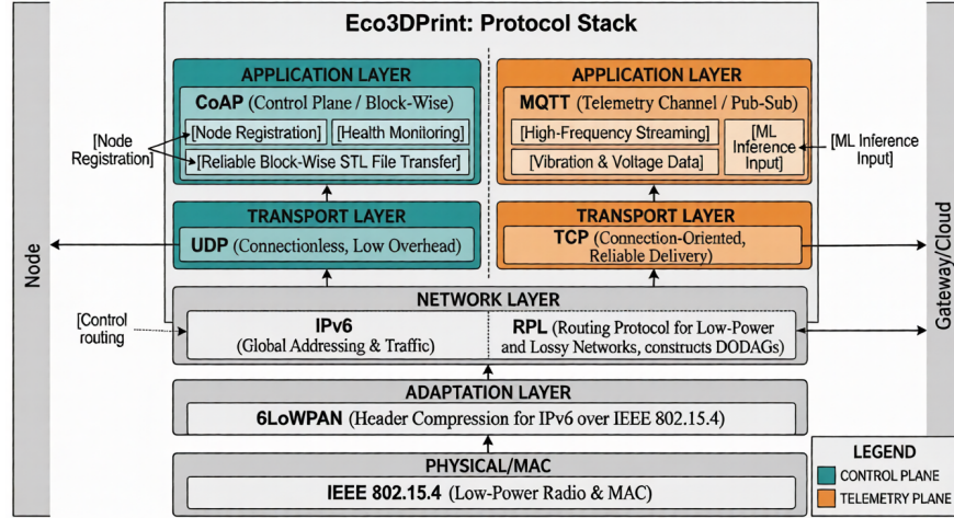
Personalized Protocol Stack of the App
