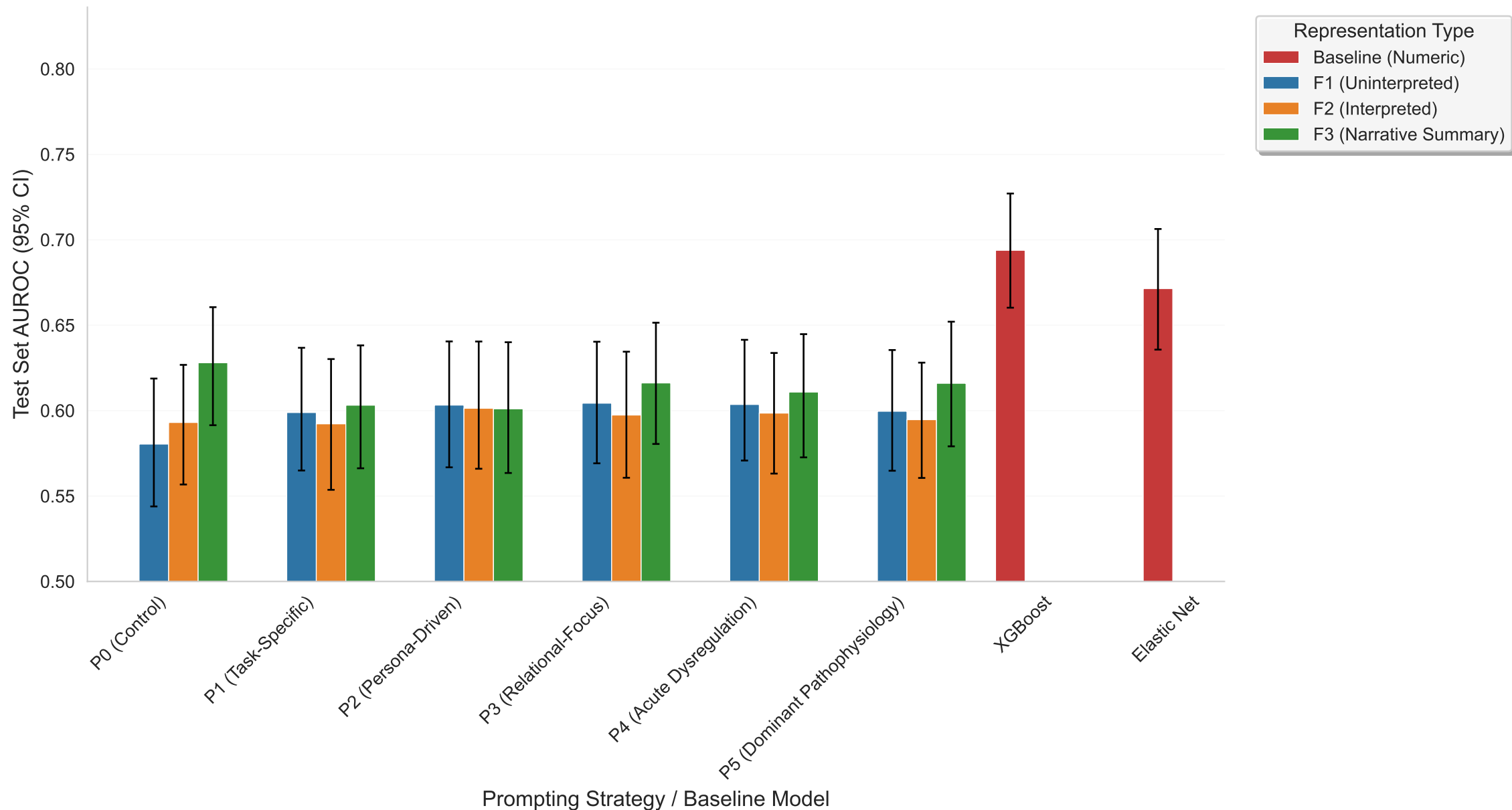
Figure 2: AUROC by Representation for Mechanical Ventilation
