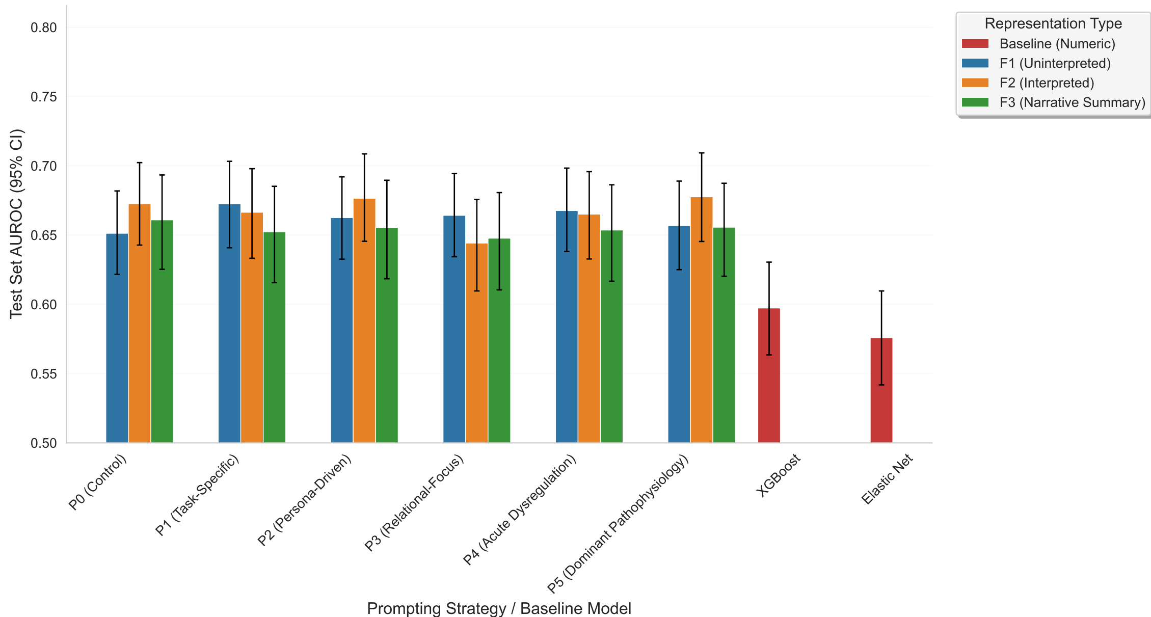
Figure 2: AUROC by Representation for 30-Day Readmission
