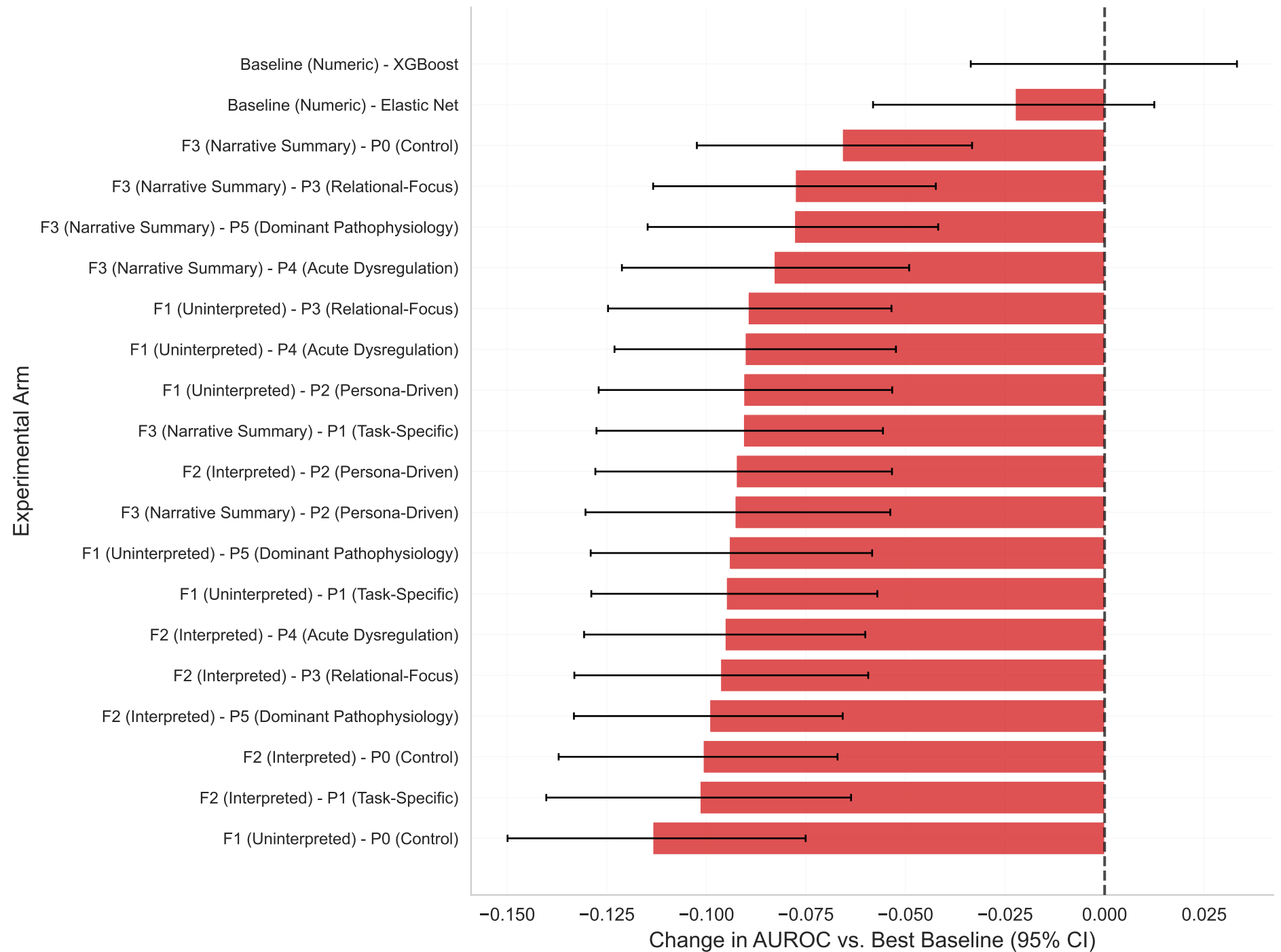
Figure 3: AUROC Improvement Over Best Baseline for Mechanical Ventilation
