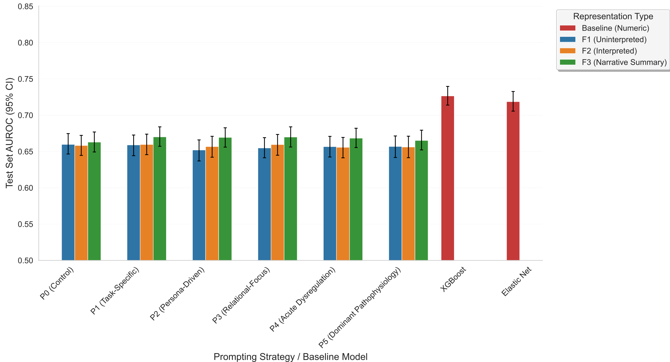
Figure 2: AUROC by Representation for Length-of-Stay > 3 Days
