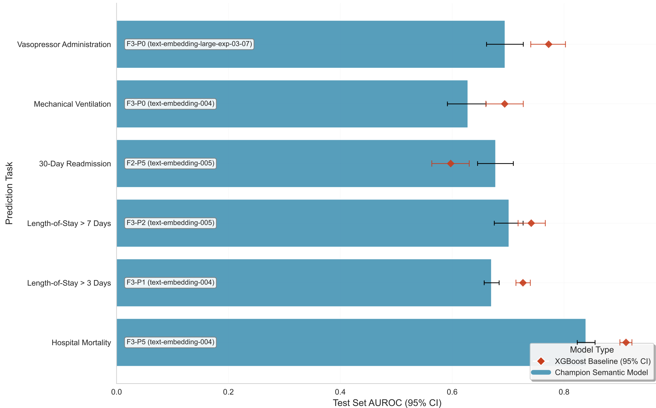
Figure 5: Champion Semantic Model vs. XGBoost Baseline by AUROC
