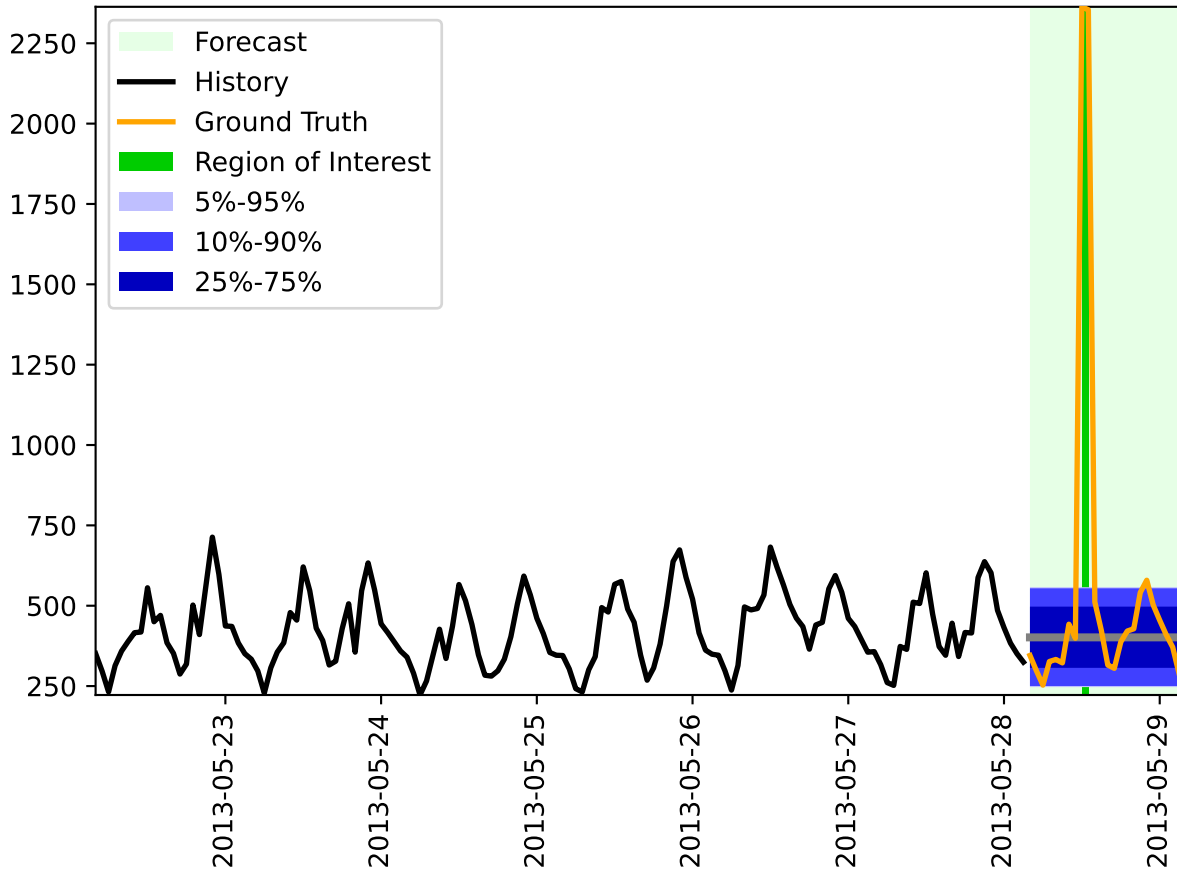
LongNewsElectricityIncreaseInPrediction task
