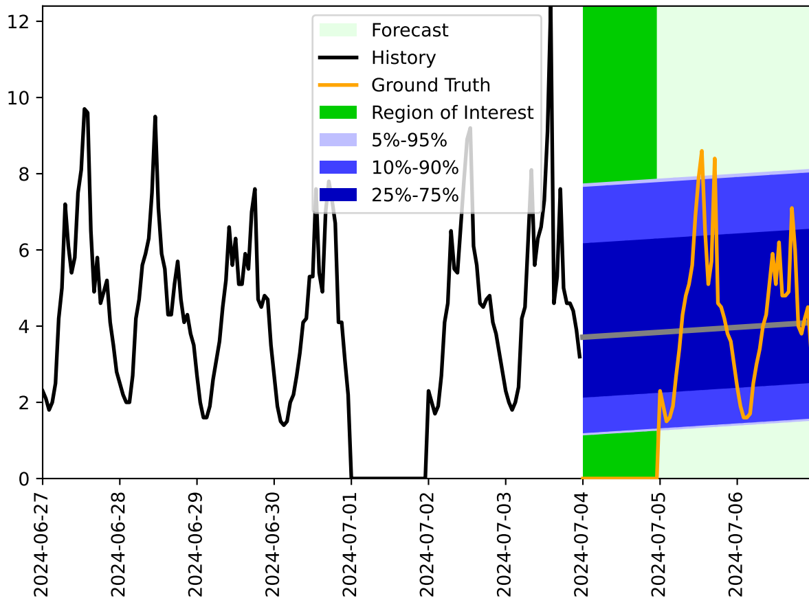
Implicit traffic forecast task with holidays in prediction window
