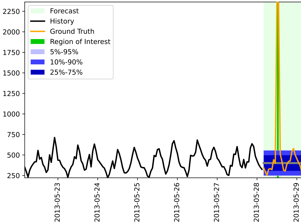
MediumNewsElectricityIncreaseInPrediction task
