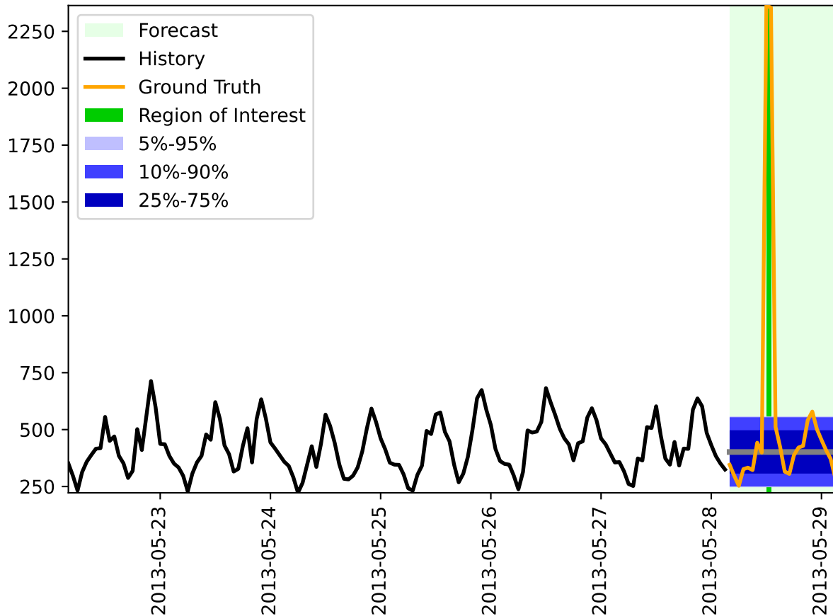
ShortNewsElectricityIncreaseInPredictionTask
