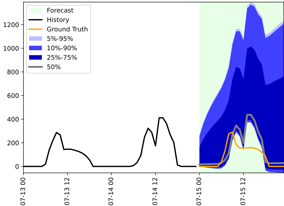
DiffuseHorizontalIrradianceFromCloudStatus
