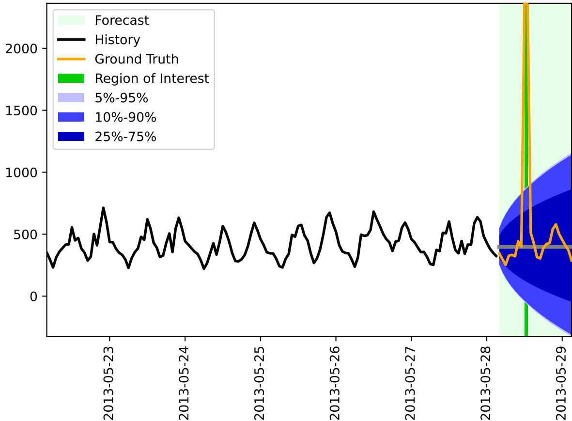
Electricity Increase Prediction With Split Context
