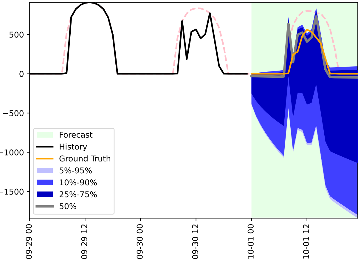
Direct Normal Irradiance from Clearsky
