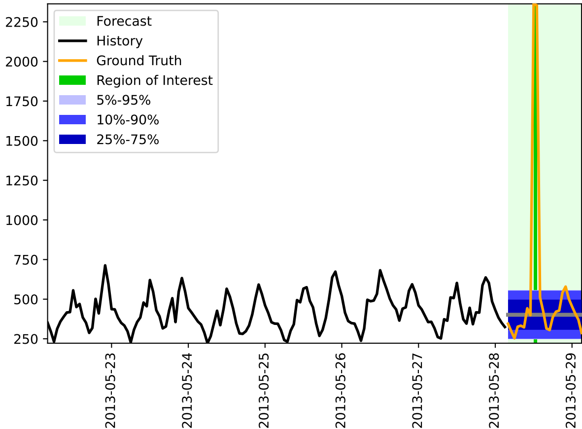
Electricity Increase in Prediction With Split Context
