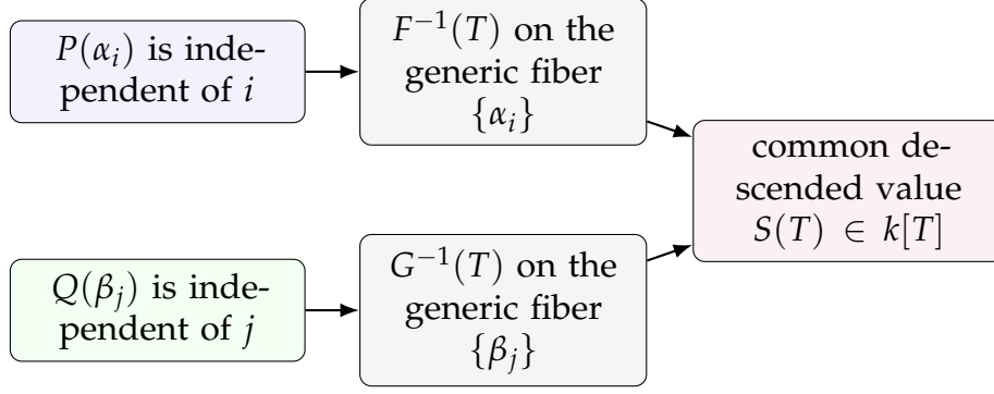
Figure 1: The separable proof: the divisibility identity forces P and Q to be constant on the generic fibers. Galois invariance gives a rational function of T , and integrality upgrades it to a polynomial.
