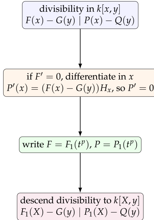
Figure 2: The Frobenius reduction step. Inseparability of an inner polynomial forces inseparability of the corresponding outer polynomial, allowing both to descend through t \mapsto t^p .
