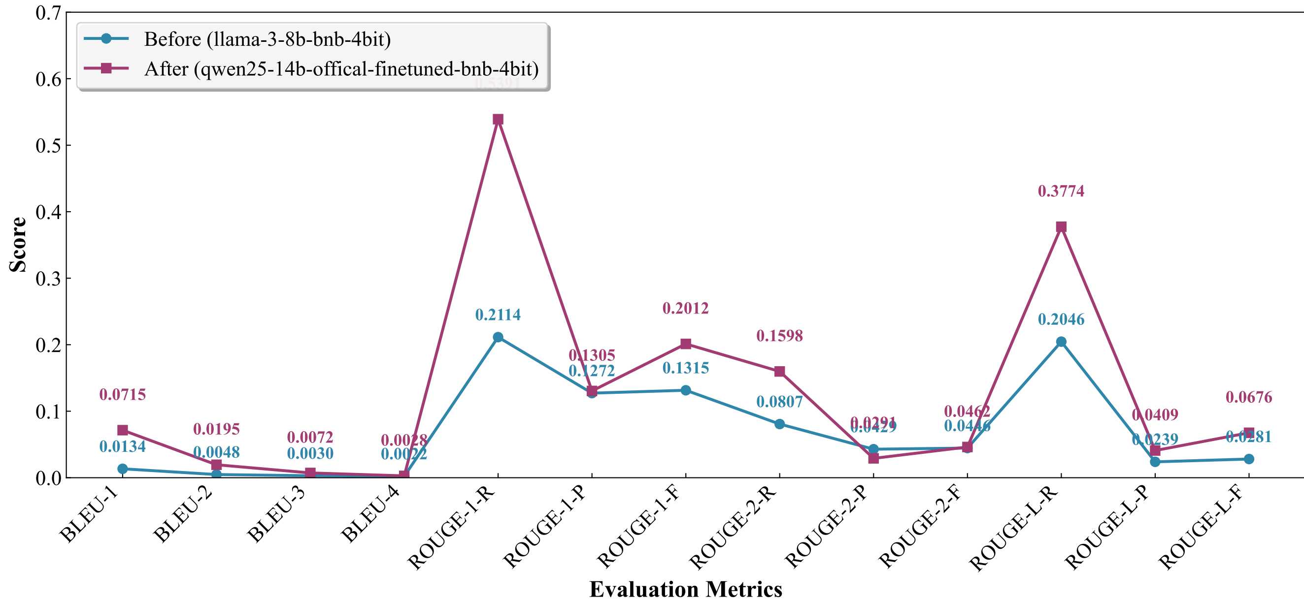
Comparison of BLEU & ROUGE Scores (Directly from MD Files)
