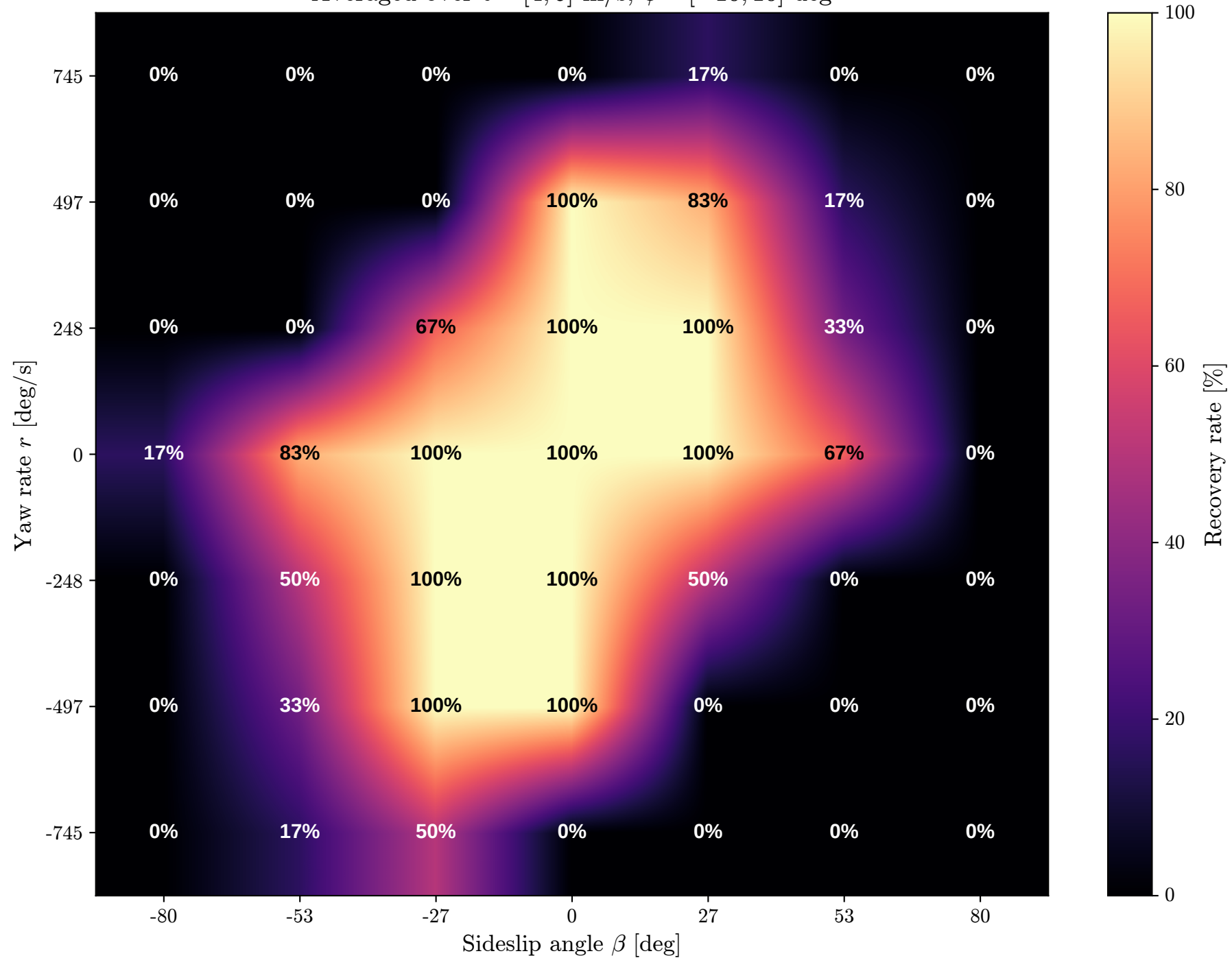
Recovery Success Rate: learned (drift) Averaged over v = [4, 5] m/s, \psi = [-10, 10] deg
