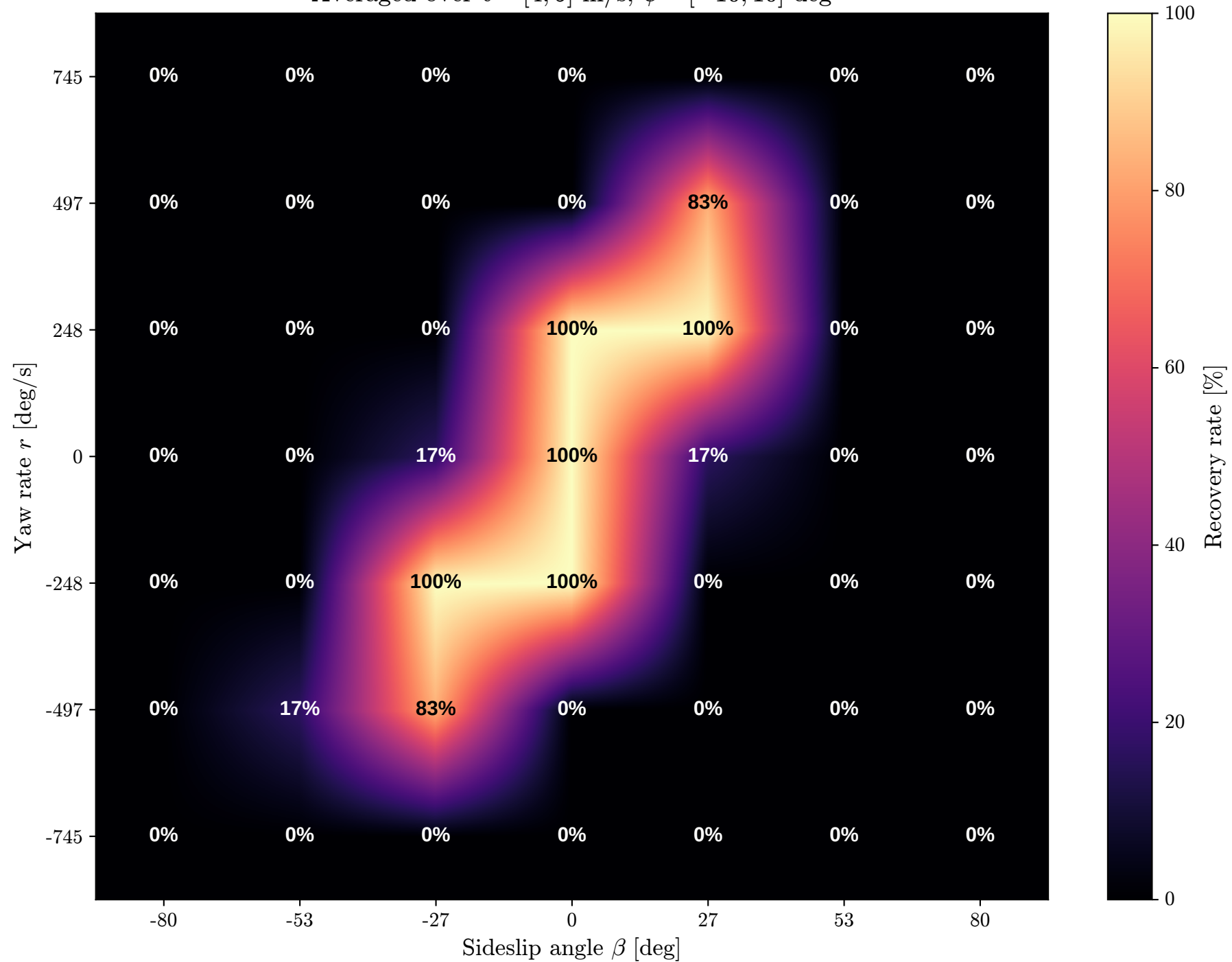
Recovery Success Rate: stmpc Averaged over v = [4, 5] m/s, \psi = [-10, 10] deg
