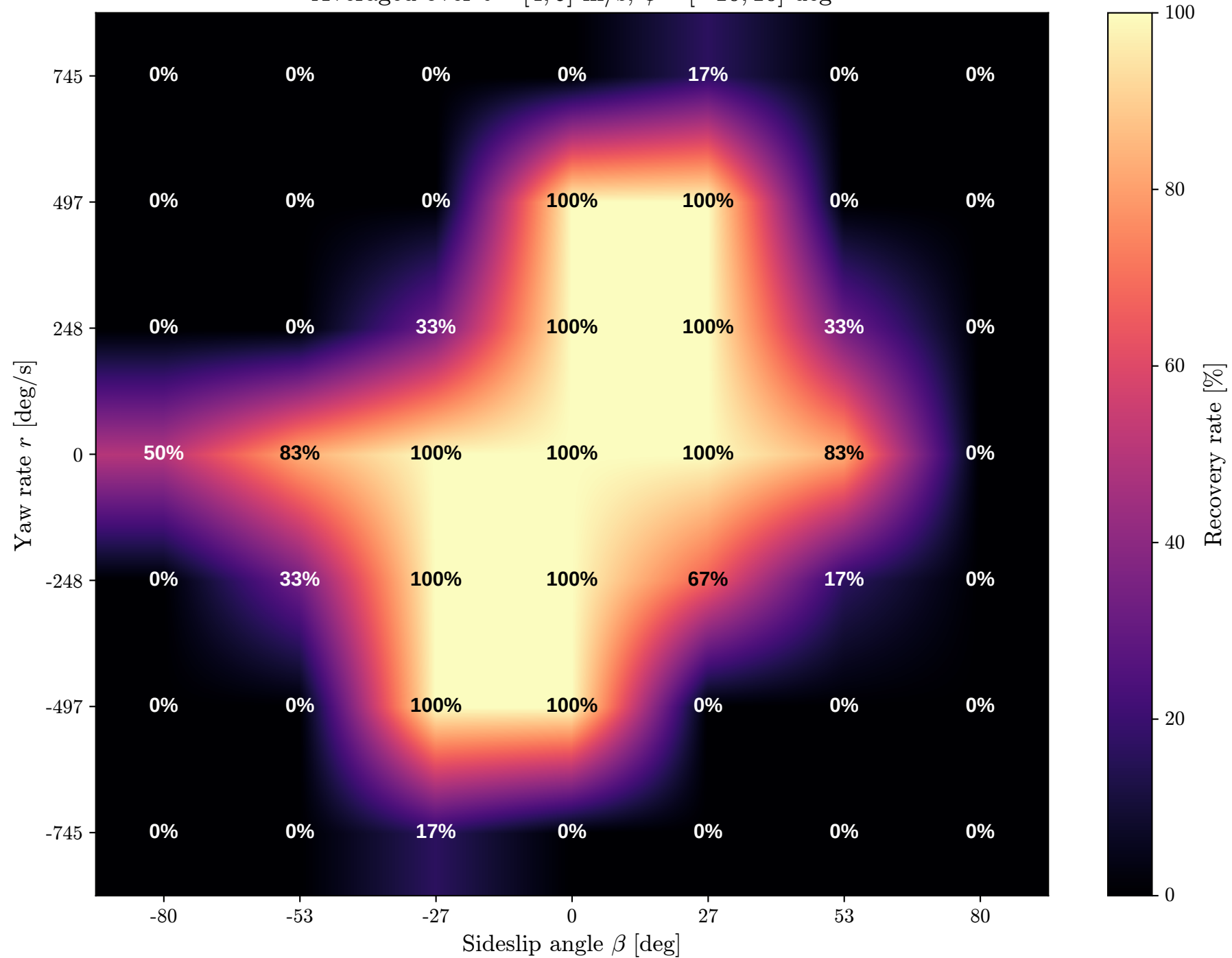
Recovery Success Rate: learned (recover) Averaged over v = [4, 5] m/s, \psi = [-10, 10] deg
