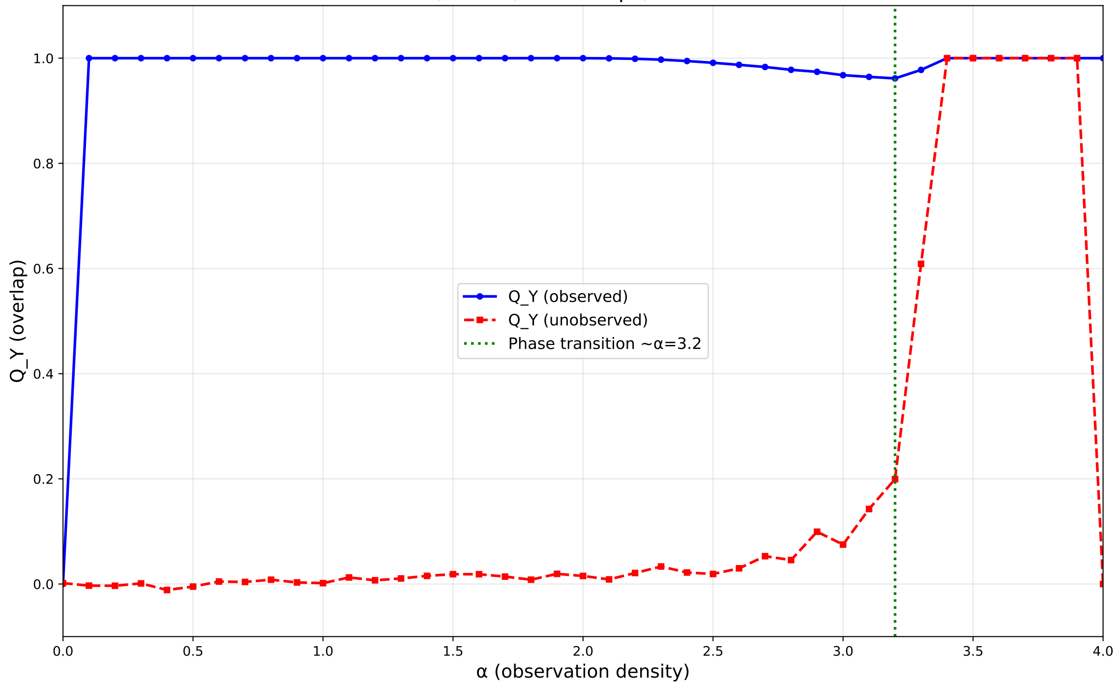
Spreading BiG-AMP Phase Transition N=200, M=50, 5000 steps, rademacher F
