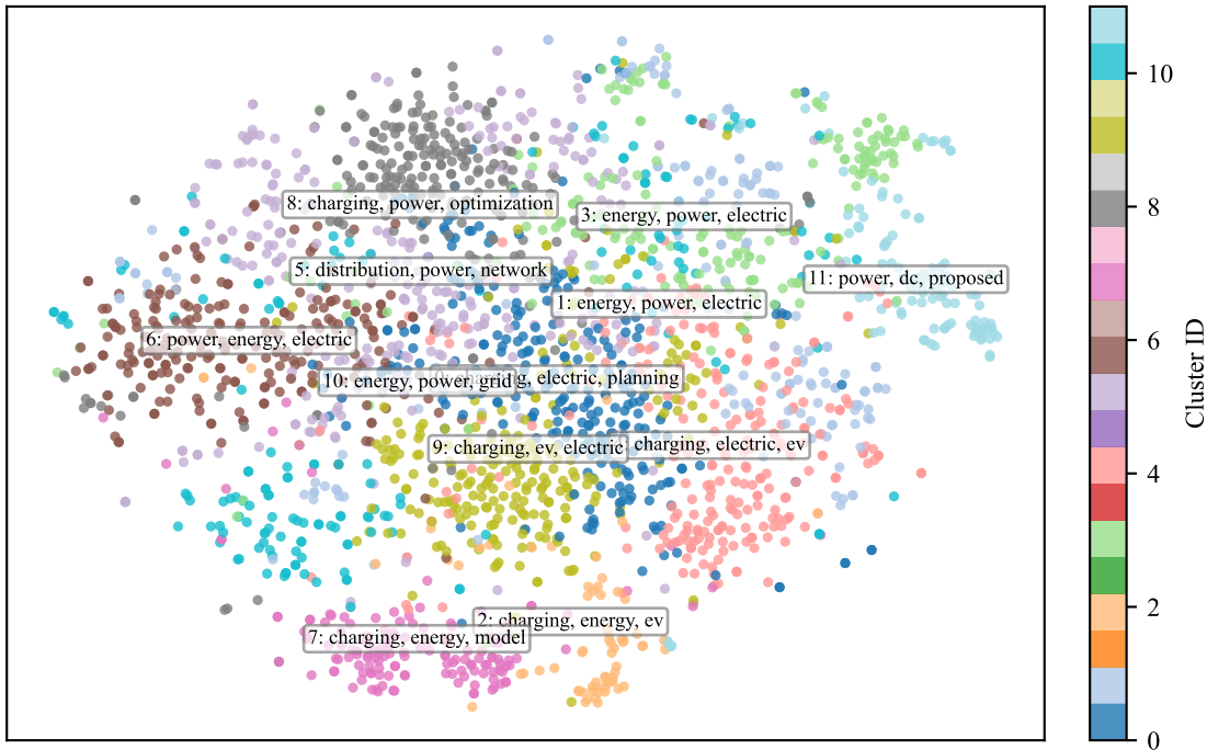
Planning corpus: t-SNE map (embeddings + KMeans)
