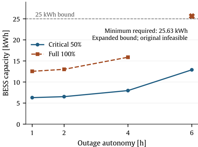
(a) BESS capacity
