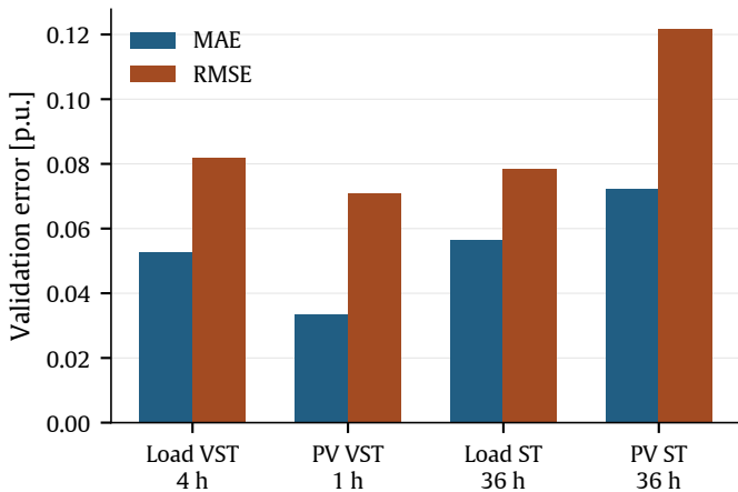
(a) MAE and RMSE
