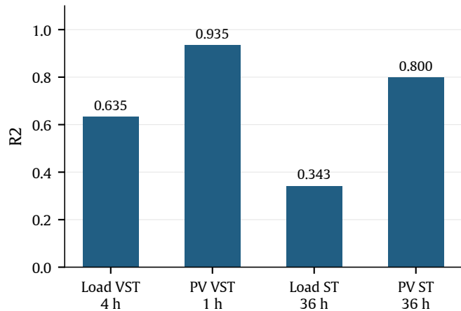
(b) Coefficient of determination
