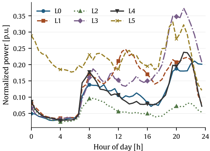
(a) Load profiles
