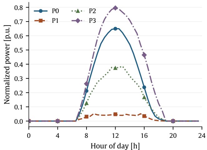
(b) PV profiles
