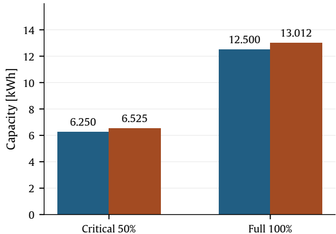
(b) BESS energy capacity
