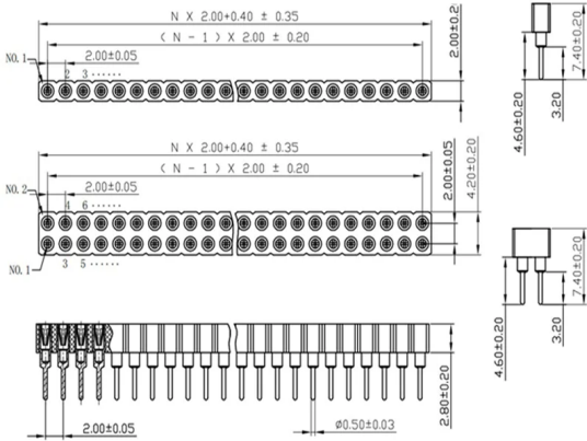
2.0MM Round Pin, Single Row/Double Row Female
