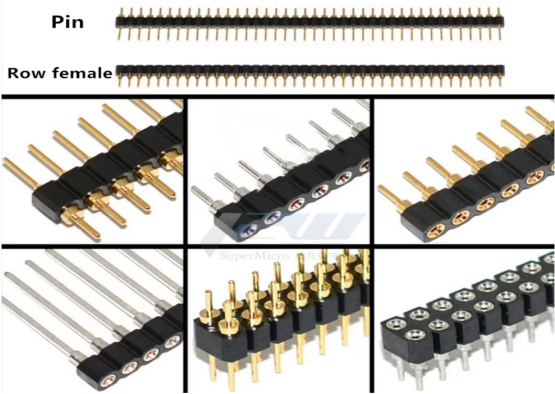
2.0MM Round Pin, Single Row/Double Row Male
