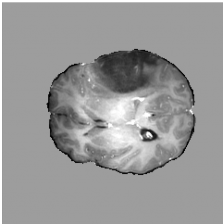
T1ce
