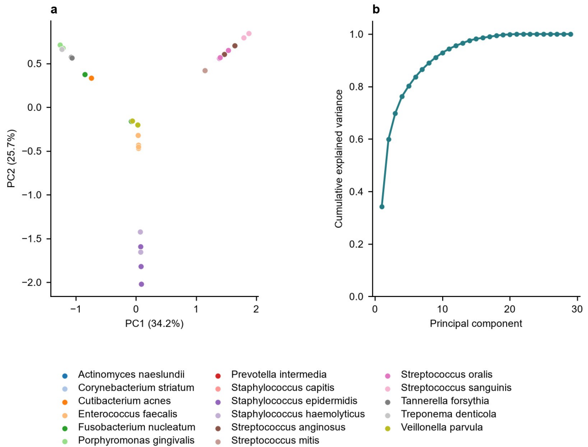
Fig. S1 Exploratory PCA of corrected annotation categories. a Assembly coordinates. b Cumulative explained variance. PC1 and PC2 explain 34.2% and 25.7%. Patterns may track taxonomy and panel construction and do not establish filler biofilm phenotypes
