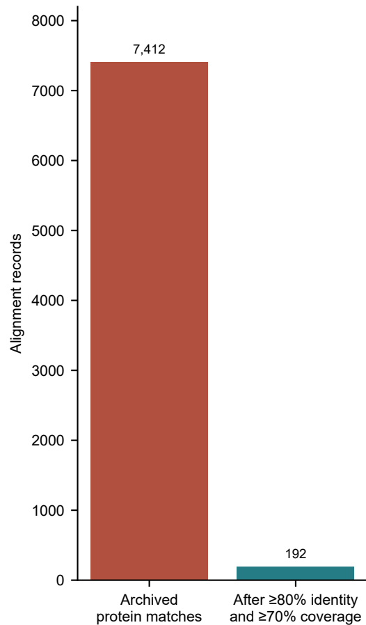
B BacMet2 threshold correction
