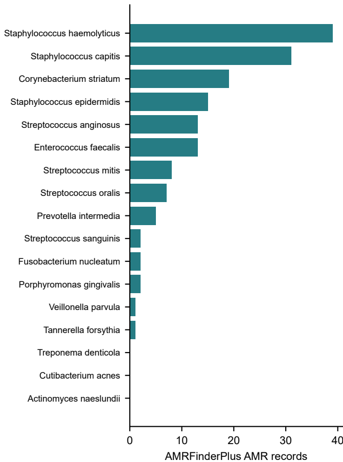
A Antibiotic resistance annotations
