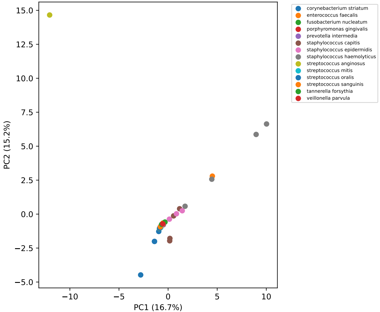
PCA based on AMR presence/absence profile
