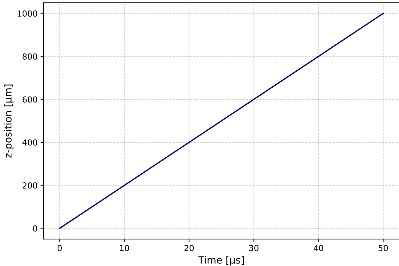
Particle motion in Penning Trap
